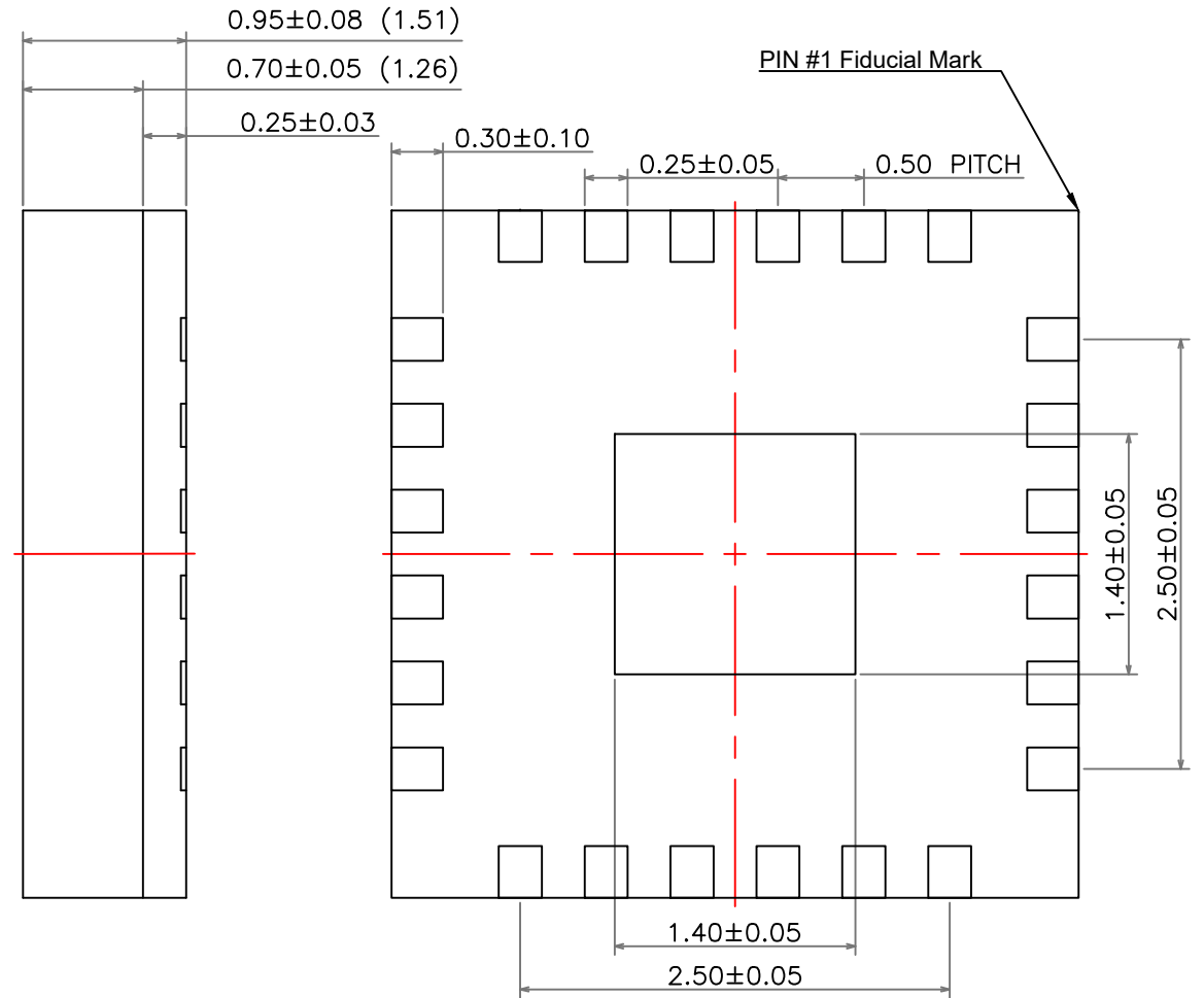
SIDE VIEW
